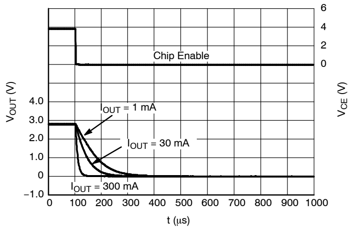
Figure 57. Shutdown, 2.8 V Version D, V_{IN} = 3.8 V
