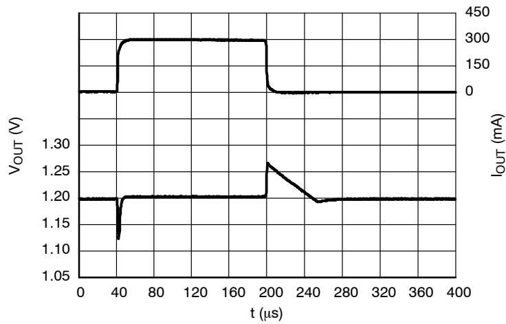
Figure 47. Load Transients, 1.2 V Version, I_{OUT} = 1 - 300 \text{ mA} , t_R = t_F = 0.5 \mu s , V_{IN} = 2.2 \text{ V}
