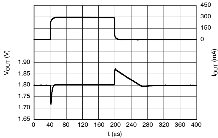
Figure 48. Load Transients, 1.8 V Version, I_{OUT} = 1 - 300 \text{ mA} , t_R = t_F = 0.5 \mu s , V_{IN} = 2.8 \text{ V}
