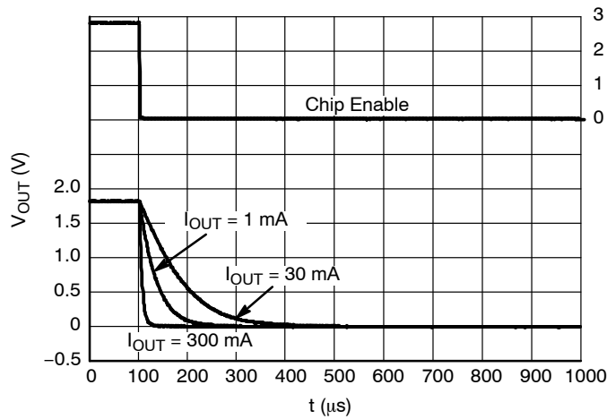
Figure 56. Shutdown, 1.8 V Version D, V_{IN} = 2.8 V
