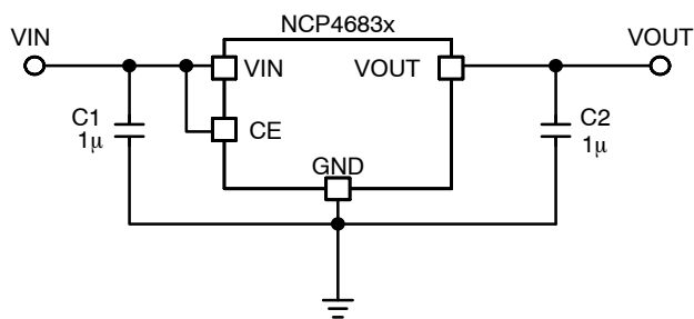
Figure 1. Typical Application Schematic
