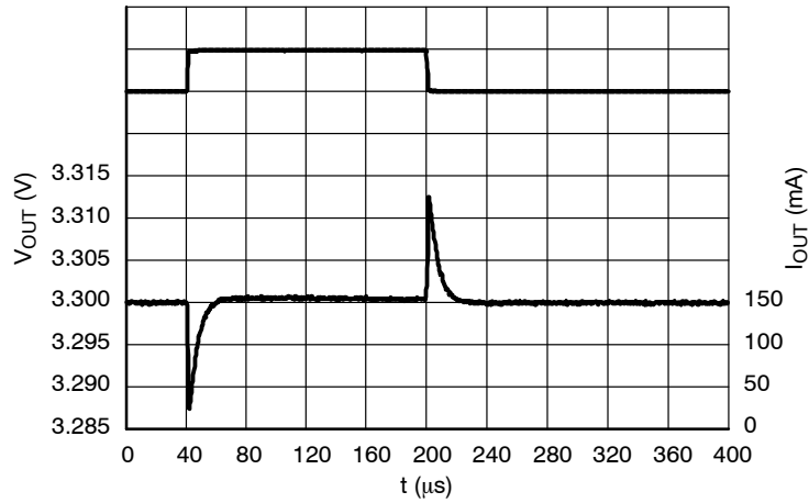
Figure 46. Load Transients, 3.3 V Version, I_{OUT} = 50 - 100 \text{ mA} , t_R = t_F = 0.5 \mu s , V_{IN} = 4.3 \text{ V}
