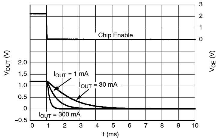
Figure 55. Shutdown, 1.2 V Version B, V_{IN} = 2.2 V
